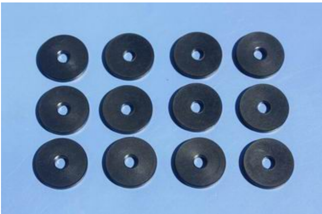
Gas engine washers for 30CC version: 12(20mm) POM washers
